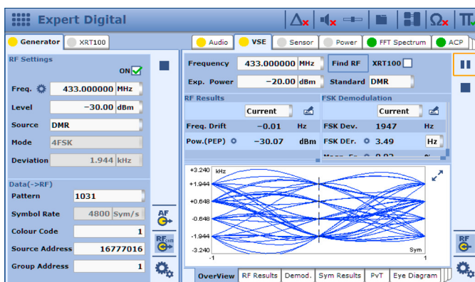
Digital signal generator for receiver tests and overview of digital measurements
