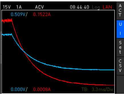
Inrush function
